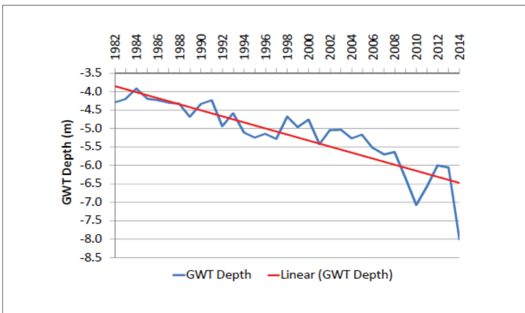
Figure 3.2: Groundwater Table depth in Northern Bangladesh 17
