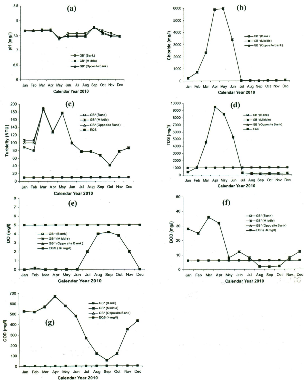
Fig. 16. Graphical presentation of pH, Chloride, Turbidity, TDS, DO, BOD and COD of Moyuri river in 2010.
